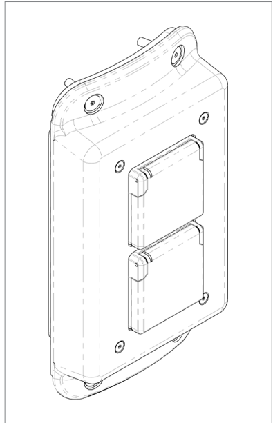
GPO/USB/OPTICAL FIBRE/ ETHERNET/HDMI (VERTICAL) ASSEMBLED VIEW
