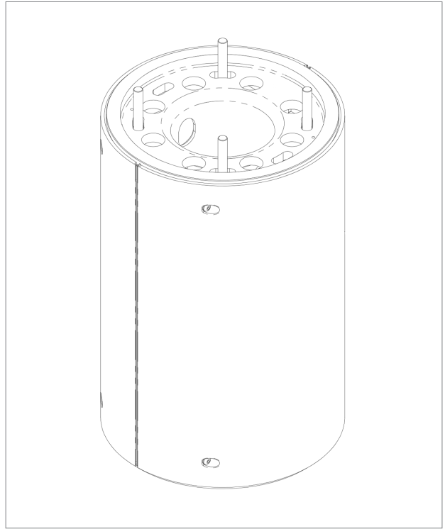
MTM ASSEMBLED VIEW
