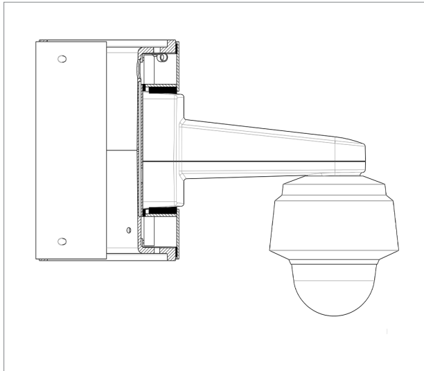
PTZ CAMERA, SIDE VIEW
