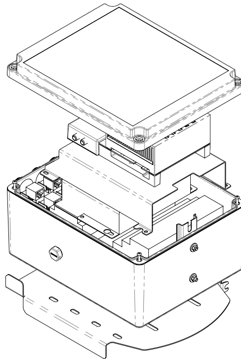
INDUSTRIAL PC, EXPLODED VIEW
